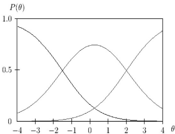
Рис. 1. A partial credit model
